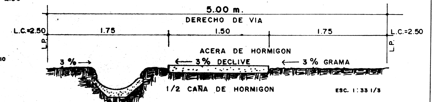
VIA PEATONAL A
